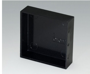
A8050160 POTTING BOXES, Vers. I PF (UL 94 V-0) black RAL 9005 50.15x50.15x15.1mm
